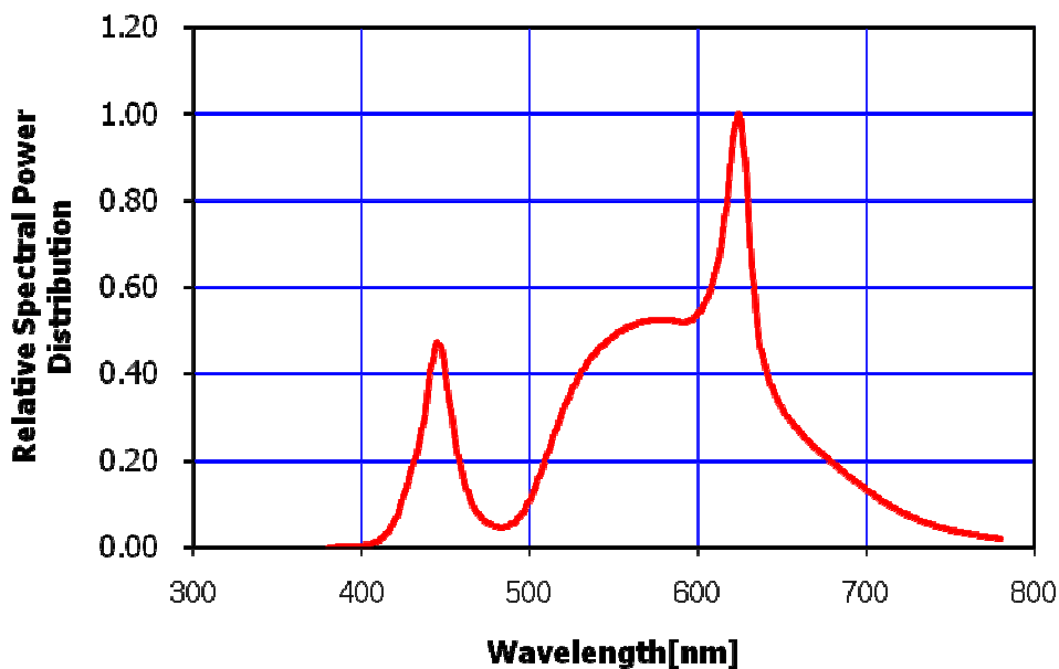
Relative Spectral Power Distribution at Ta=25°C
