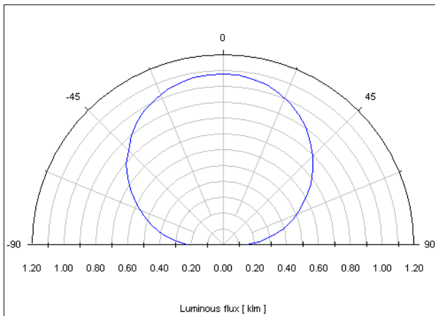
Radiation Pattern
